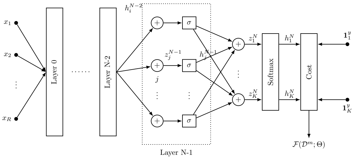
Figure 2.3: Representation of a Multi-Layer Perceptron (MLP) or Feed-Forward (FF) network as a computation graph. The classification cost for the m -th training example \mathcal{D}^m = \{\mathbf{x}, y\} is also shown.
