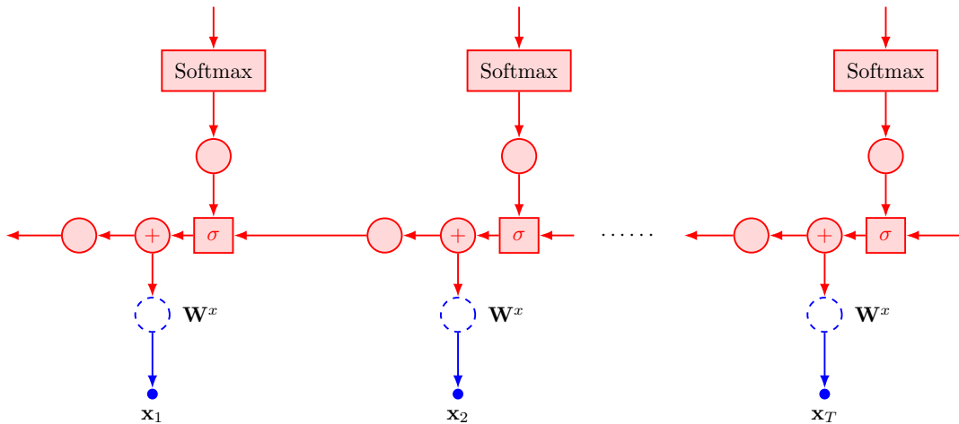
Figure 3.2: Forward-pass (blue) and backpropagated error (red) to the input layer of an RNN. Note that a copy of the error is sent to each output of each sum node (+)
