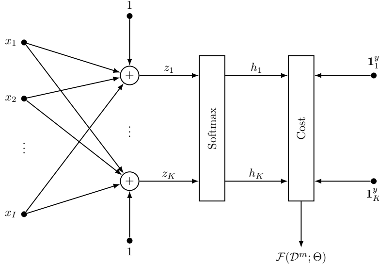
Figure 2.1: Representation of a log-linear model as a computation graph: a composition of linear and non-linear transformations. The classification cost for the m -th training example \mathcal{D}^m = \{\mathbf{x}, y\} is also shown. Note \mathbf{1}^y is an indicator vector of size K with a one in position y and zeros elsewhere.
