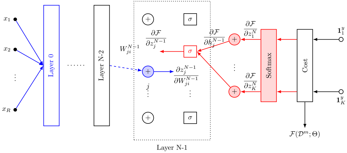
Figure 2.4: Forward-pass (blue) and Backpropagation (red) calculations to estimate the gradient of weight W_{ji} at layer N - 1 of a MLP.
