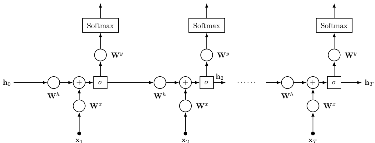
Figure 3.1: The simplest RNN can be seen as replicating a single hidden-layer FF network T times and passing the intermediate hidden variable h_t across different steps. Note that all nodes operate over vector inputs e.g., x_t \in \mathbb{R}^I . Circles indicate matrix multiplications.
